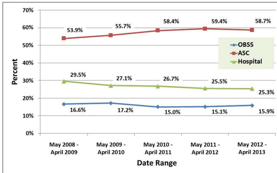
Figure 1. Yearly trends for usage of different types of facilities where cosmetic surgeries were performed. ASC, ambulatory surgery center; OBSS, office-based surgical suite.
