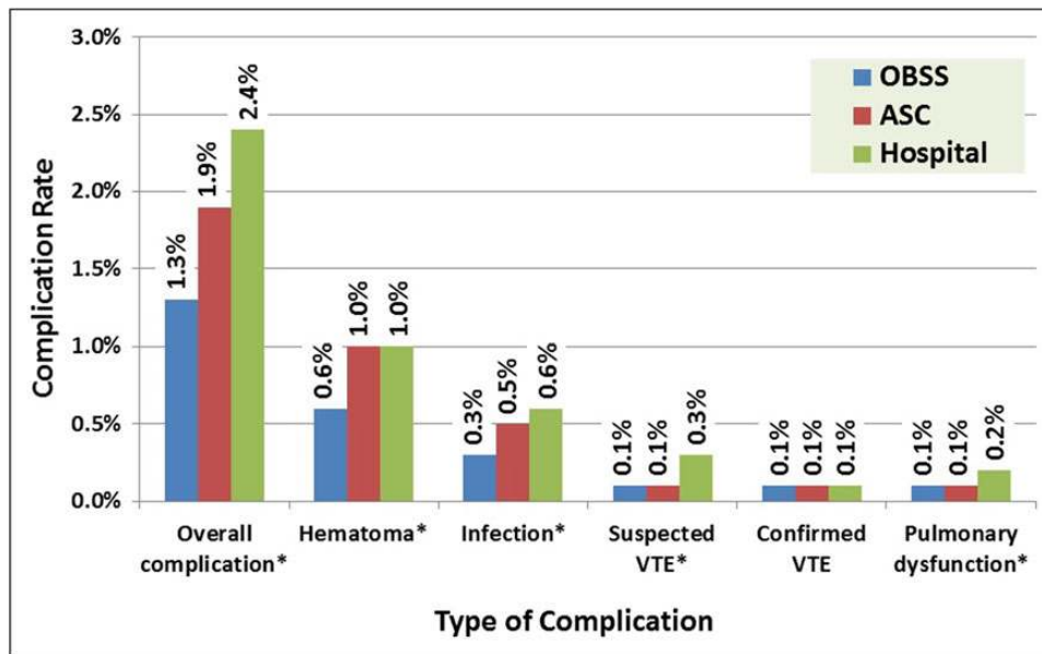
Figure 2. Overall and individual complication rates by type of facility. ASC, ambulatory surgery center; OBSS, office-based surgical suite; VTE, venous thromboembolism.
